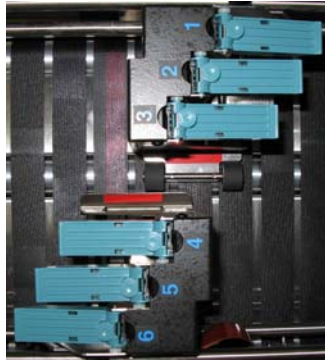
SIX PRINTHEADS
